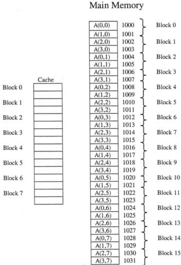
Figure 6.11 Array elements in the main memory
